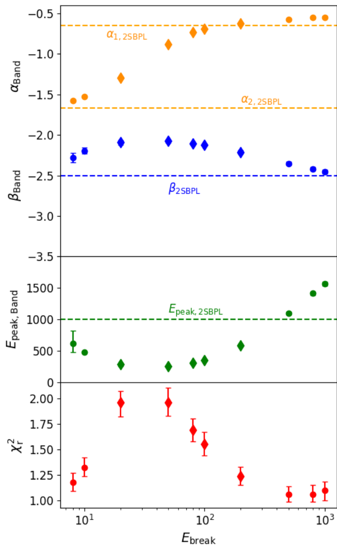
Fig. 2. Band function parameters as a function of the position of the energy break E_{\text{break}} of the 2SBPL function. Each plot shows the parameters of the Band function fitted to a series of spectra simulated assuming the 2SBPL function whose parameter values are marked by the horizontal dashed lines. Top: low-energy slope \alpha_{\text{Band}} (orange symbols) and high-energy slope \beta_{\text{Band}} (blue symbols). Middle: energy peak E_{\text{peak, Band}} (green symbols). Bottom: fit \chi_r^2 (red symbols). Left: spectrum characterized by a S/N \sim 21 (fluence \sim 3.5 \cdot 10^{-4} erg \text{cm}^{-2} ). Right: spectrum characterized by S/N \sim 2.7 (fluence \sim 3.5 \cdot 10^{-5} erg \text{cm}^{-2} ). Data are represented as circles when the best-fitting model is Band and as diamonds when the best-fitting model is 2SBPL.
