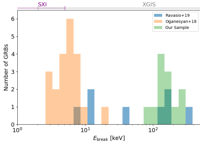
Fig. 4. Energy distribution of the spectral breaks identified in prompt spectra of GRBs, from the results of Oganesyan et al. (2018) , Ravasio et al. (2019) , and this work. The horizontal lines indicate the observational energy range of the instrumentation aboard THESEUS.
